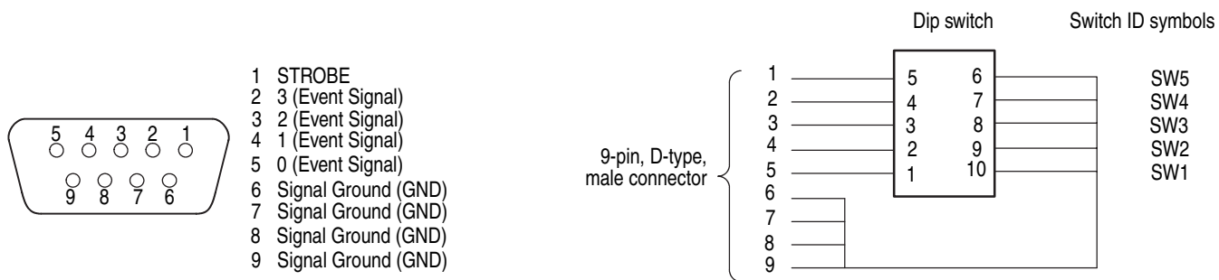
Figure B-37: EVENT IN connector pins and signals and ground closure connector
